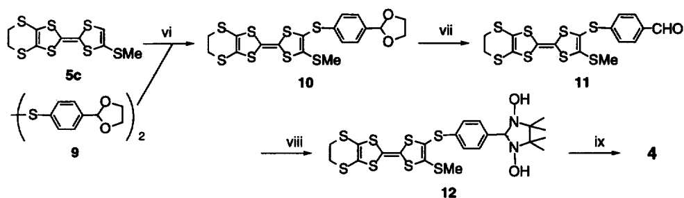
Scheme 2. Reagents and conditions: (vi) (1) LDA, THF, -70^\circ C , 1h, (2) 9 , THF, -70^\circ C to rt, overnight, 55%; (vii) TsOH- H_2O , CHCl_3 -acetone, overnight, 90%; (viii) (C(CH_3)_2(NHOH))_2 , cat. (C(CH_3)_2(NHOH))_2 \cdot H_2SO_4 , benzene-MeOH, reflux, 12h, 50%; (ix) PbO_2 , K_2CO_3 , THF, rt, 40 min.
