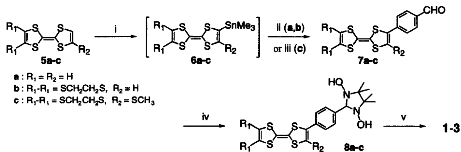
Scheme 1. Reagents and conditions: (i) (1) LDA, THF, -70^\circ C , 1h, (2) Me_3SnCl , THF, -70^\circ C , 2h; (ii) BrPhCHO, Pd(PPh_3)_2Cl_2 , toluene, reflux, 8h, a:50%, b:60%; (iii) IPHCHO, Pd(PPh_3)_4 , toluene-1M Na_2CO_3 aq, reflux, 20h, 55%; (iv) (C(CH_3)_2(NHOH))_2 , cat. (C(CH_3)_2(NHOH))_2 \cdot H_2SO_4 , CH_2Cl_2 -hexane(2:1), reflux, overnight, a:85%, b:35%, c:90%; (v) PbO_2 , K_2CO_3 , THF, rt, 40 min.
