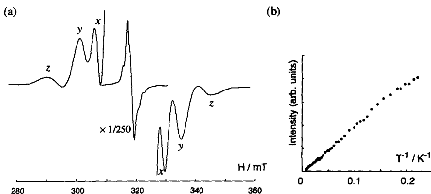
Figure 1. (a) ESR spectrum of iodine-doped 3. (b) Temperature dependence of triplet signal intensity of 3 •• .
