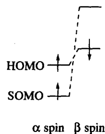
Figure 2. UHF description of the spin polarization of HOMO caused by SOMO in a spin-polarized donor.
